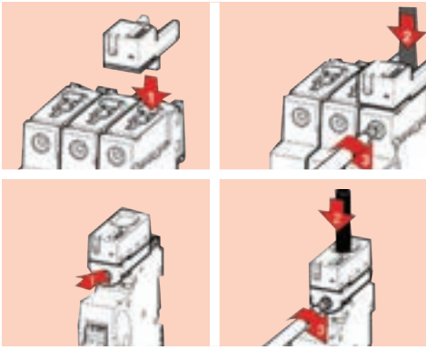
Easy MCB-mount sensors saves up to 30% of installation time
