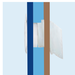
Reduced spigot length for back-to-back installation with a through-wall fan
