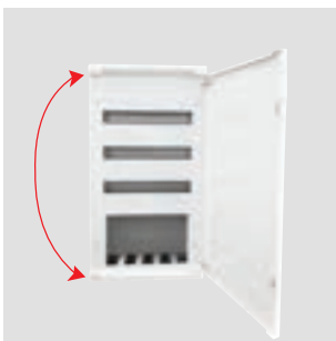
Boards are able to be rotated
