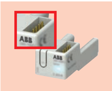
One sensor for all currents DC, AC, or mixed (up to 160A)
